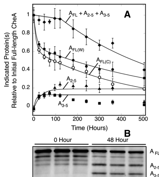
Figure 4. Timecourse of full-length CheA decay and the appearance of CheA proteolytic fragments. A) Triplicate, membrane-bound arrays reconstituted from serine receptor, CheA kinase and CheW coupling protein were incubated at 22 °C for 504 h (21 days). At the indicated time points a sample was removed from each triplicate and pelleted to separate array-bound and supernatant CheA. Pelleted samples were resolved on SDS gels and Western blotted with polyclonal anti-CheA antibody. The timecourses of full-length CheA decay were similar, generally within error, when monitored by Western blotting (filled circles) and Coomassie staining (open circles). In addition to the full-length CheA band, two smaller bands were observed building up in the array Western blots. These bands are observed at the molecular weights expected for CheA lacking the P1 domain (triangles, P2–P3–P4–P5) and for CheA lacking the P1–P2 domains (squares, P3–P4–P5). The sum of the Western blot densities for full-length CheA, P2–P3–P4–P5, and P3–P4–P5 were also determined (diamonds). All data are relative to the initial level of full-length CheA. B) Sample Western blot showing the full-length CheA band and the two degradation products initially and after 48 h.
