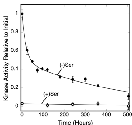
Figure 2. Kinase activity as array ages. Serine receptor-containing E. coli membranes were reconstituted in vitro with Cysless CheA kinase and CheW coupling protein to yield triplicate arrays and then were incubated at 22 °C for 504 h (21 days). At the indicated time points a sample was removed from each triplicate and mixed with CheY and ATP to measure the array kinase activity (closed circles). An identical sample was mixed with attractant serine to measure attractant regulation (open circles). The data were best fit either with the double exponential decay of eq 1 (curve, no serine) or with a straight line (serine). Error bars indicate the standard deviation of each triplicate mean.
