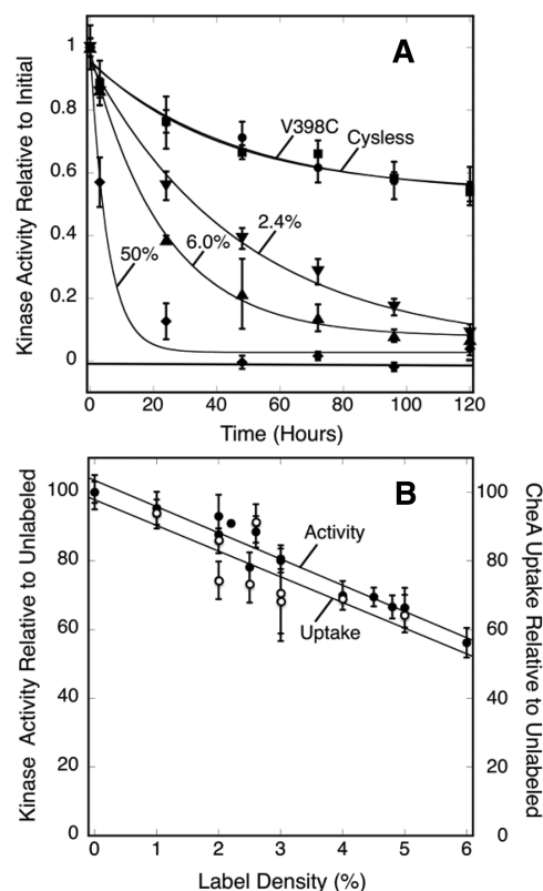
Figure 8. Examining the relationship between defects, stability, and assembly. A) Membrane-bound receptor populations containing the single Cys mutant V398C were labeled with the indicated levels of 5-(iodoacetamido)fluorescein to introduce local defects and then reconstituted arrays were formed with CheA and CheW. Triplicate samples were incubated at 22 °C for 120 h (5 days), and at the indicated time points a sample was removed from each triplicate and its kinase activity was determined. Error bars indicate the standard deviation of each triplicate mean. Normal attractant regulation was confirmed on the initial, second, and fifth day of the experiment by addition of 1 mM serine (open symbols). B) The initial time point samples generated for different defect densities in (A) were also analyzed for their CheA incorporation (open circles) and kinase activities (closed circles) just after array reconstitution. Error bars indicate the standard deviation of each triplicate mean. Data in (A) were best fit by eq 4 consisting of a single exponential decay term to model the fast quasi-stable population and a constant term to approximate the amplitude of the ultrastable population.
