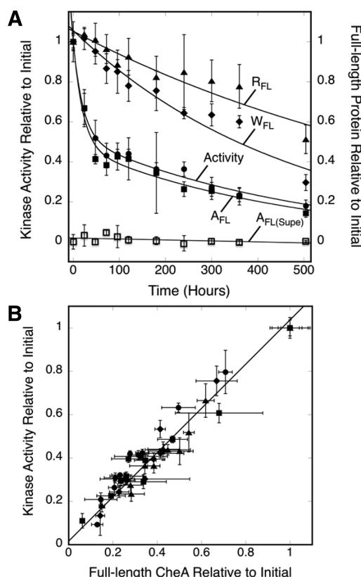
Figure 3. Comparing the kinetics of kinase activity loss and protein loss. A) Triplicate, membrane-bound arrays reconstituted from serine receptor, CheA kinase and CheW coupling protein were incubated at 22 °C for 504 h (21 days). At the indicated time points a sample was removed from each triplicate and mixed with CheY and ATP to determine the kinase activity of the array (circles). Another sample was pelleted to separate and quantitate array bound CheA (closed squares) and CheA in the supernatant (open squares). Pelleted samples were also utilized to quantitate array bound, full-length CheW (diamonds) and full-length Tsr (triangles). The data were best fit with the double exponential decay of eq 1 yielding the indicated best fit curves (kinase activity and pellets) or were best fit with a straight line (supernatant). B) Plot investigating the correlation between the average kinase activity and level of full length CheA measured at a given time point for each triplicate in (A), as well as 3 other independent experiments like (A). Error bars indicate the standard deviation of the triplicate mean for each parameter.
