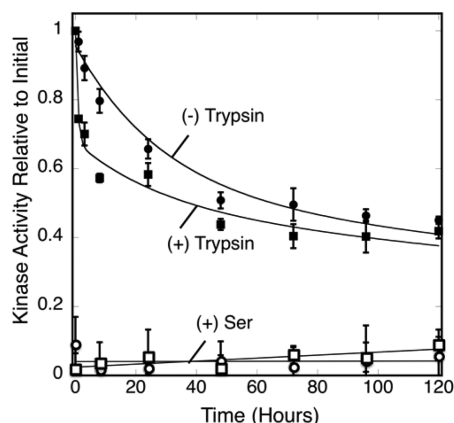
Figure 5. Kinetic comparison of endogenous and exogenous proteolysis. Triplicate, membrane-bound arrays reconstituted from serine receptor, CheA kinase and CheW coupling protein were incubated at 22 °C for 120 h (5 days) under normal conditions (filled circles) or with 3 nM trypsin (filled squares). At the indicated time points a sample was removed from each triplicate, and its kinase activity was determined in the absence (filled circles, squares) or presence (open circles, squares) of attractant serine. Error bars indicate the standard deviation of each triplicate mean. The (-) trypsin data (curve) were best fit by eq 2, a variation of the double exponential decay of eq 1 where the lifetime ( \tau_f and \tau_s ) was fixed (29 and 460 h) to the averages obtained from Figure 1, eq 1. The (+) trypsin data (curve) were best fit by eq 3, a variation of eq 2 that contained a third exponential term that was not fixed to any predetermined value.
