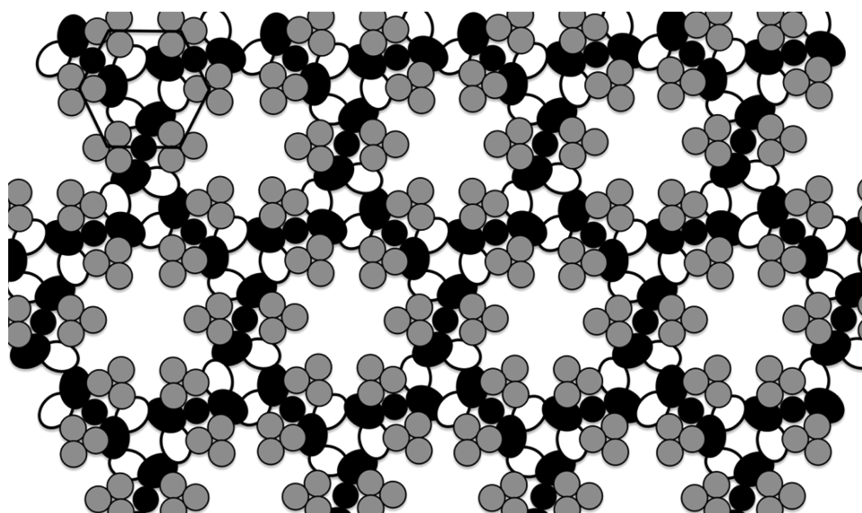
Figure 1. Working model of the core bacterial chemosensory array. 20,31,32 Receptor trimer-of-dimers (gray) are arrayed in a hexagonal pattern with one trimer at each vertex. Homodimers of the multidomain CheA His kinase (black) pack between the long edges of adjacent trimers and also contact CheW (white oval). CheW and the structurally homologous P5 domain of CheA (black oval) interact with one another in a head to tail fashion forming an interconnected ring. This basic hexagonal unit is propagated throughout the array, forming a network of interconnected rings.
