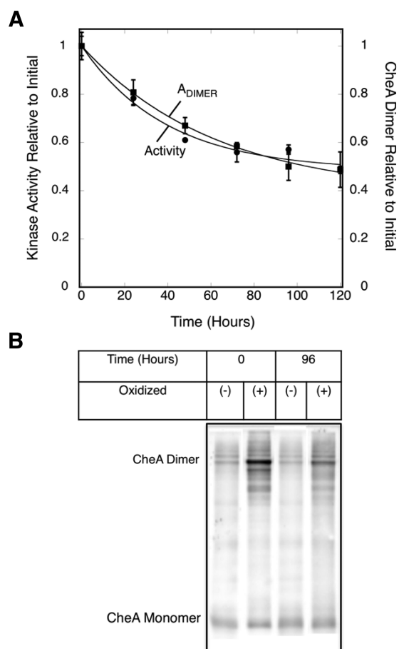
Figure 6. Decay timecourse of full length CheA dimers detected by disulfide cross-linking. Triplicate, membrane-bound arrays reconstituted from serine receptor, E311C CheA kinase and CheW coupling protein were incubated at 22 °C for 120 h (5 days). A) At the indicated time points a sample was removed from each triplicate and incubated with 6 mM CuCl 2 for 10 min to covalently link the subunits of the E311C CheA homodimer. Samples were pelleted, resolved on SDS gels, and Western blotted with polyclonal anti-CheA yielding the decay timecourse of the full length CheA dimer (squares). For comparison, the decay timecourse of Cysless kinase activity is also plotted (circles). Error bars indicate the standard deviation of each triplicate mean. B) Western blot showing the oxidative cross-linking of E311C CheA in reconstituted arrays to yield covalent homodimer.
